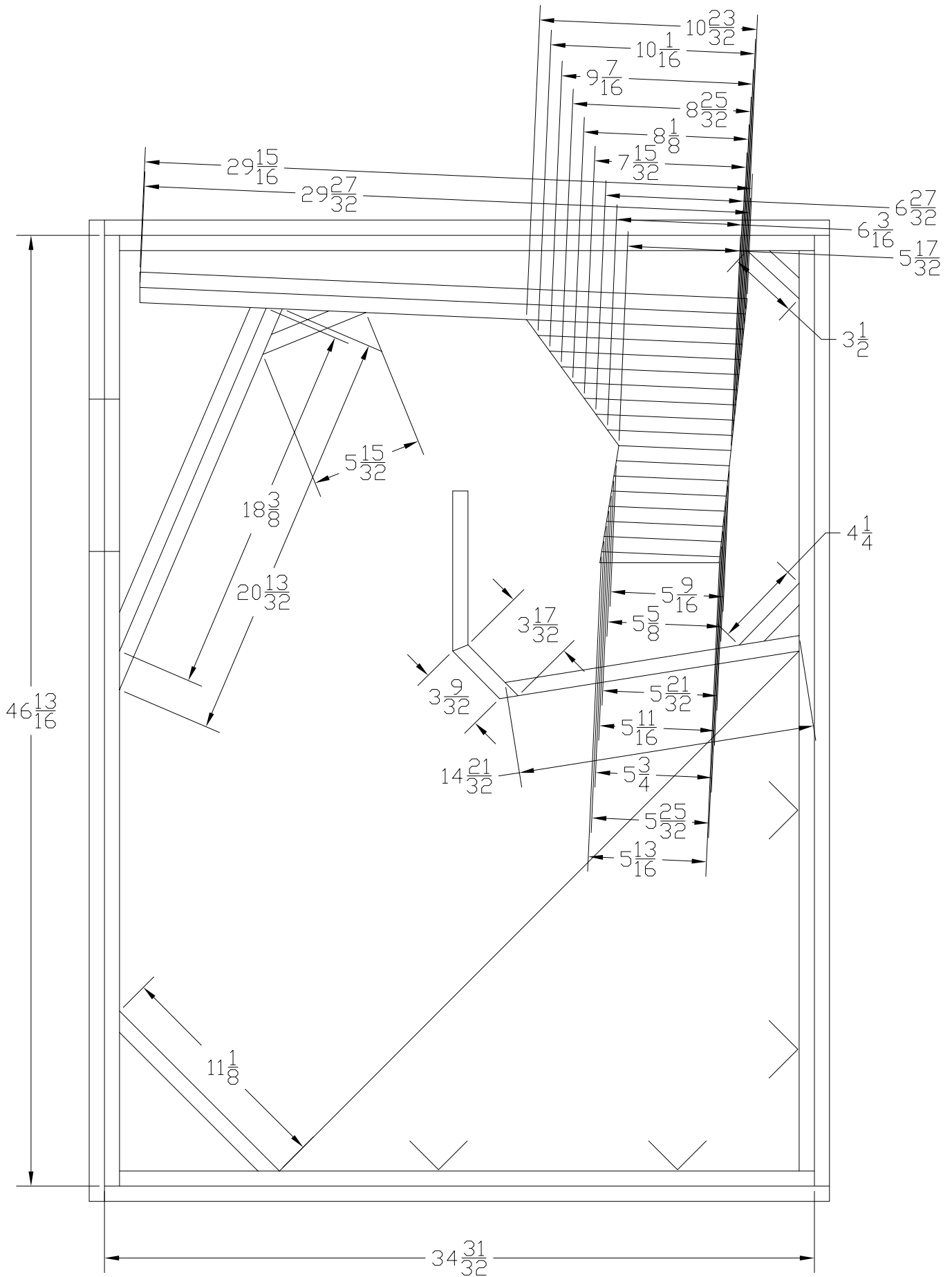
Side panel dim's: 46-13/16 \times 34-31/32
